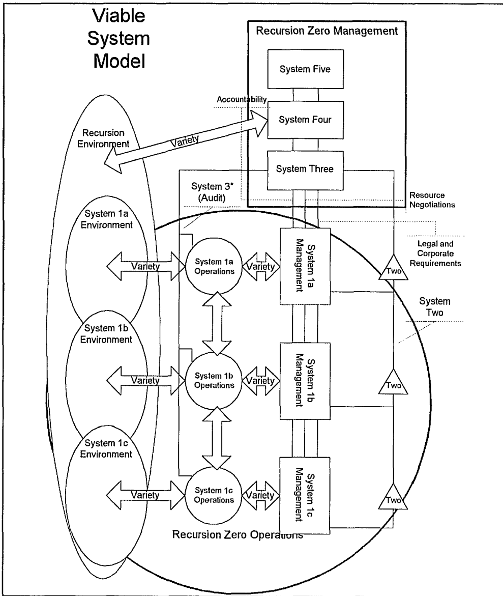
Figure 5.5 The VSM - Recursions Zero and One.
